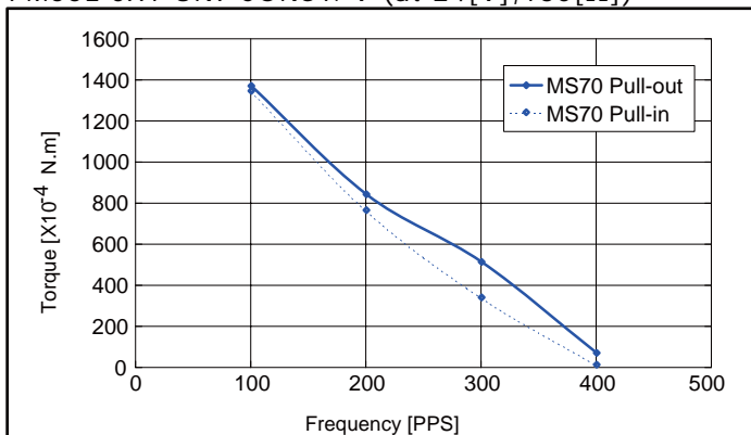
PM55L-0X1 UNI-CONST. V (at 24[V], 130[Ω])
