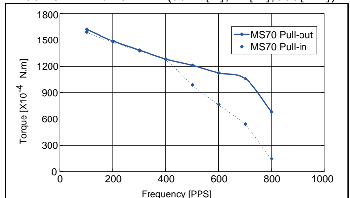
PM55L-0X1 BI-CHOPPER (at 24[V], 7.1[Ω], 500[mA])
