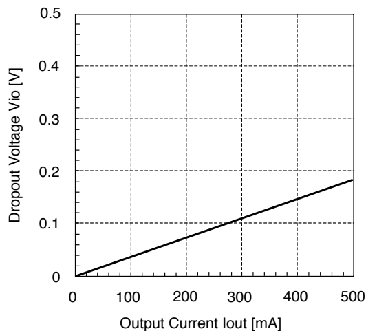
■ Dropout Voltage
