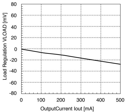
■ Load Regulation
