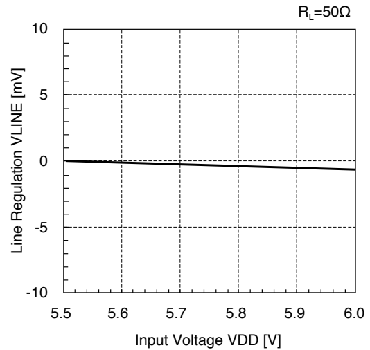
■ Line Regulation
